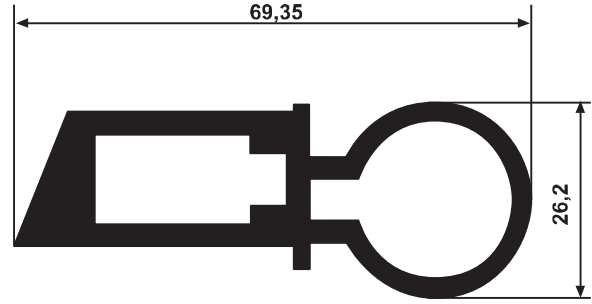
YG 1181 1,541 kg/m
